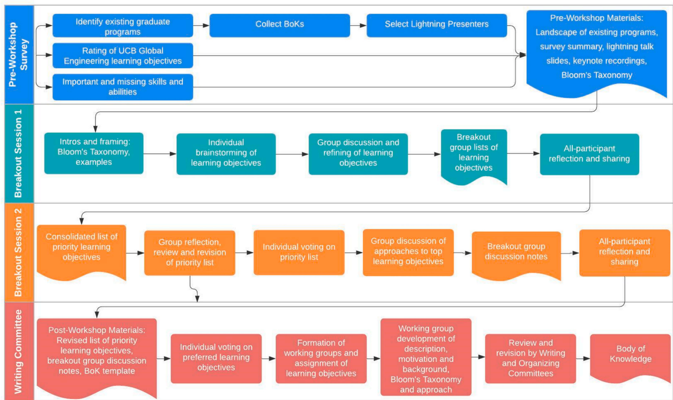
Fig. 2. Methodology.
