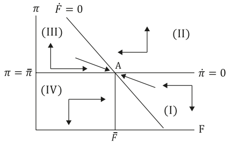
Figure 1: Saddle point solution
