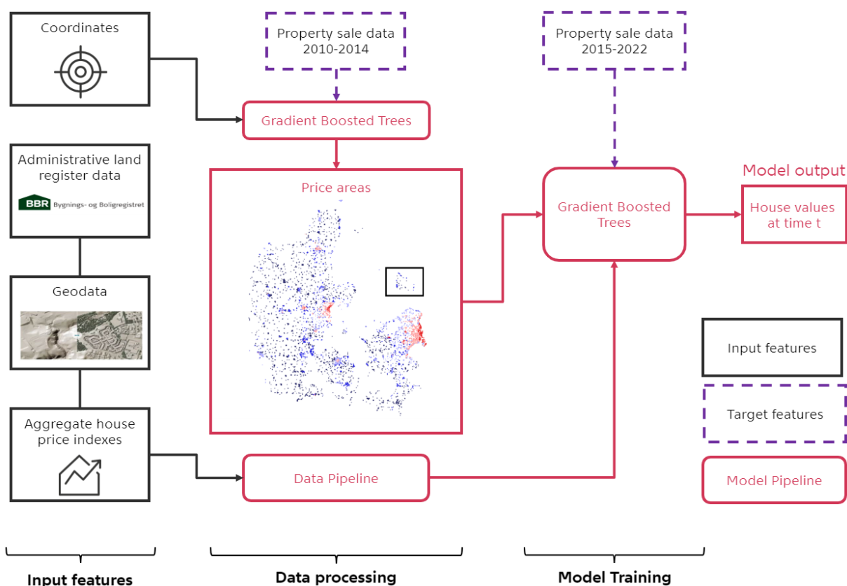
The full valuation model consists of a data pipeline, an auxiliary price area model and a final house value model
