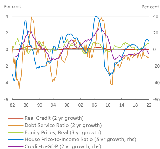
High comovement makes identification difficult
