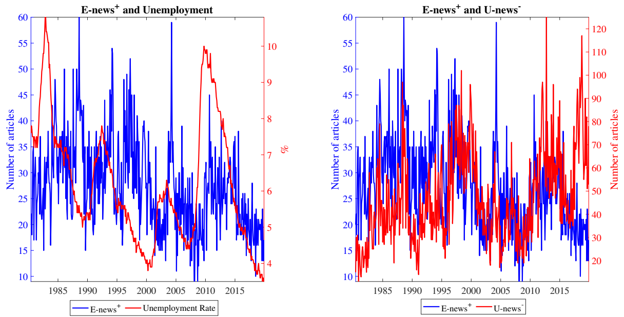
Figure 10: Alternative measure of good news - E\text{-news}^+
