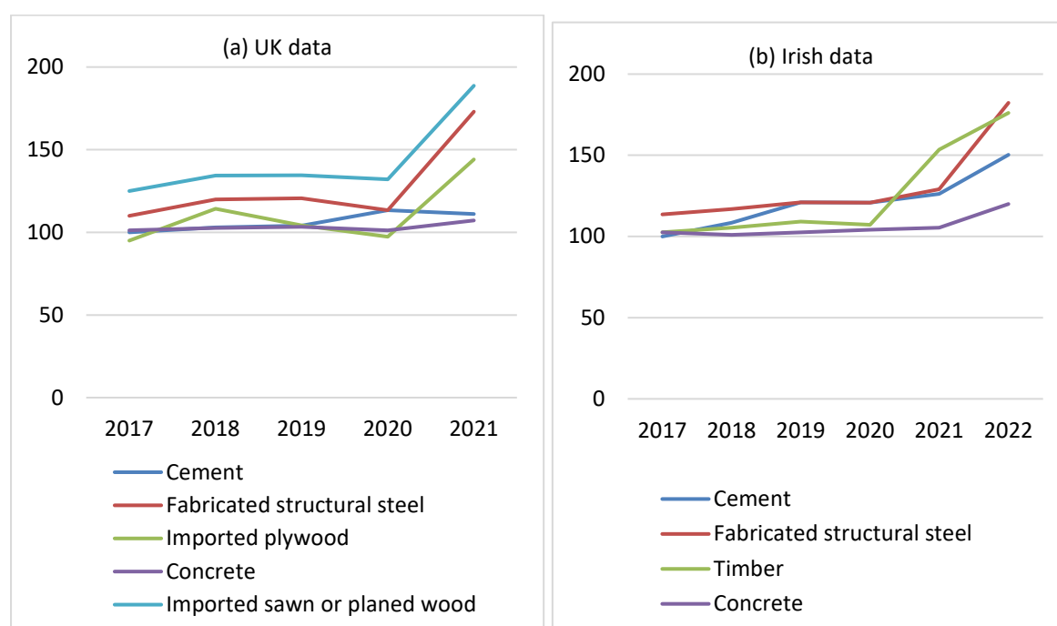
FIGURE 4.1 PRICES OF MATERIALS IN THE UK AND IRELAND (NOMINAL INDEX 2015 = 100)
