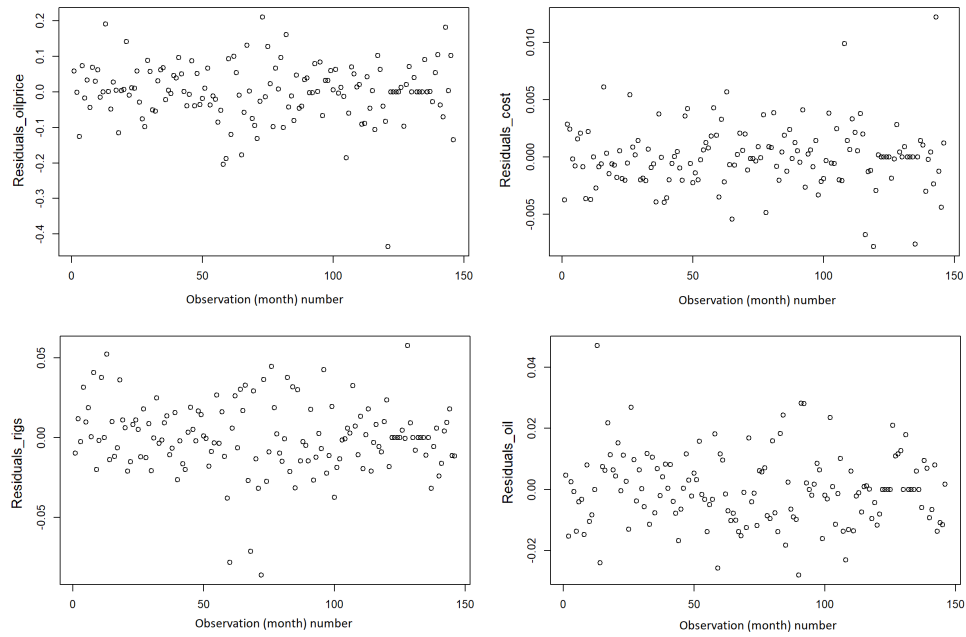
Figure 12: Regression residuals.
