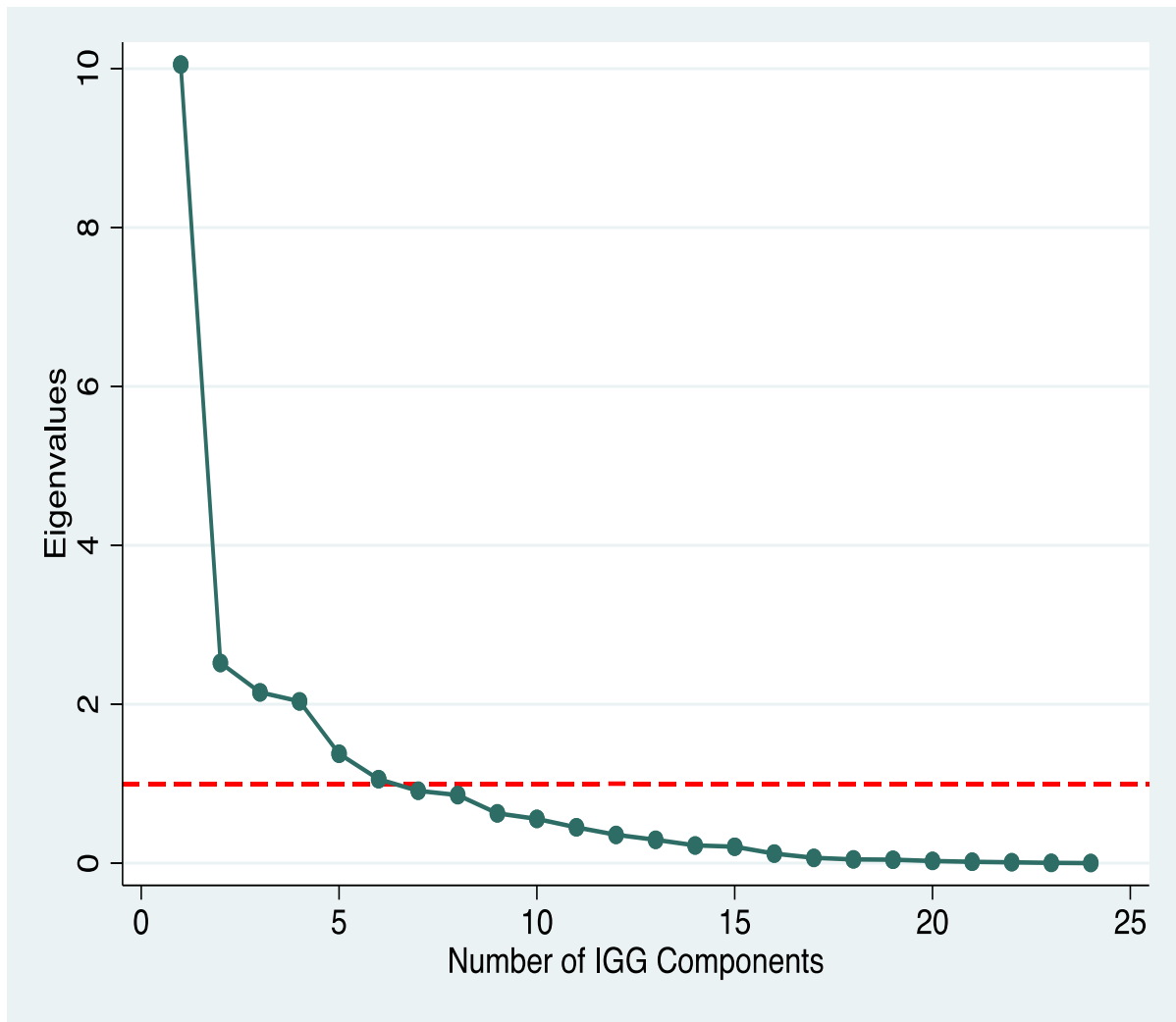
Figure A.1: Screeplot of IGG Components
