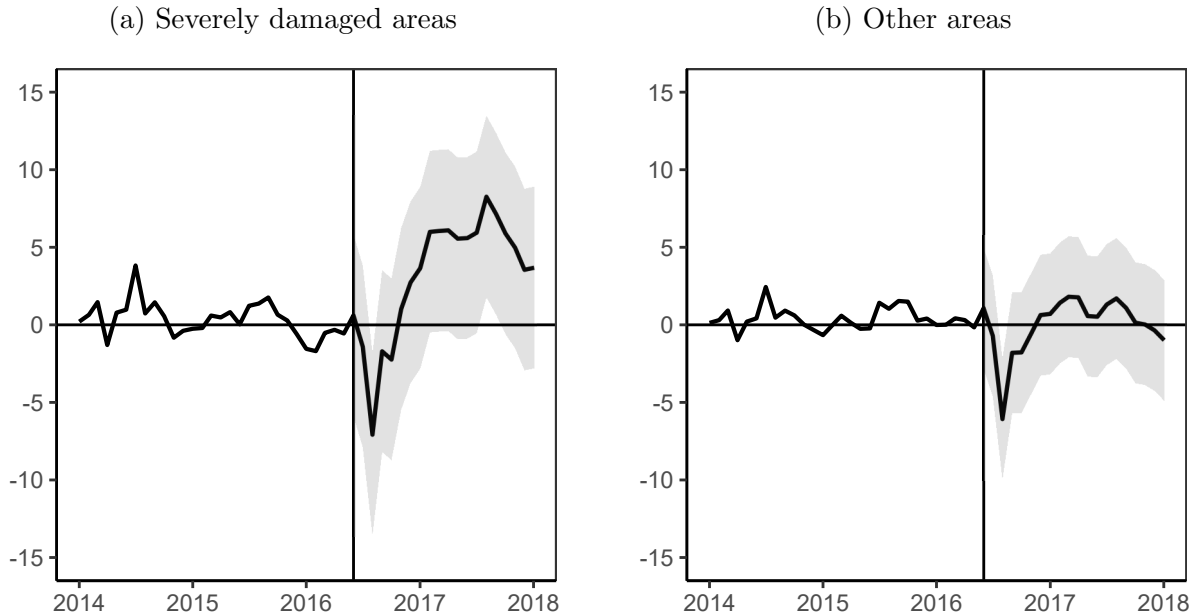
Figure C.4: Gap between actual and synthetic credit scores
