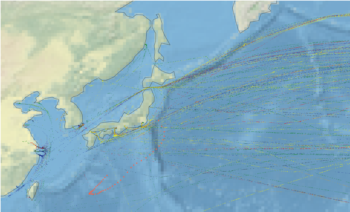
Figure 3: Typhoon Lionrock, late August, 2016
