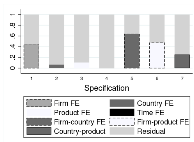
(b) Alternative specifications with one set of fixed effects at a time
