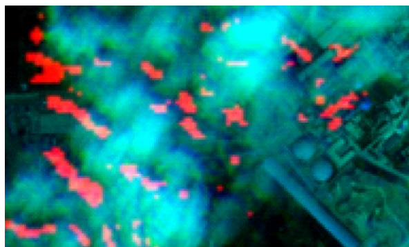
Figure 4. Effects of clouds on heat detection (“hot” pixels in red)
