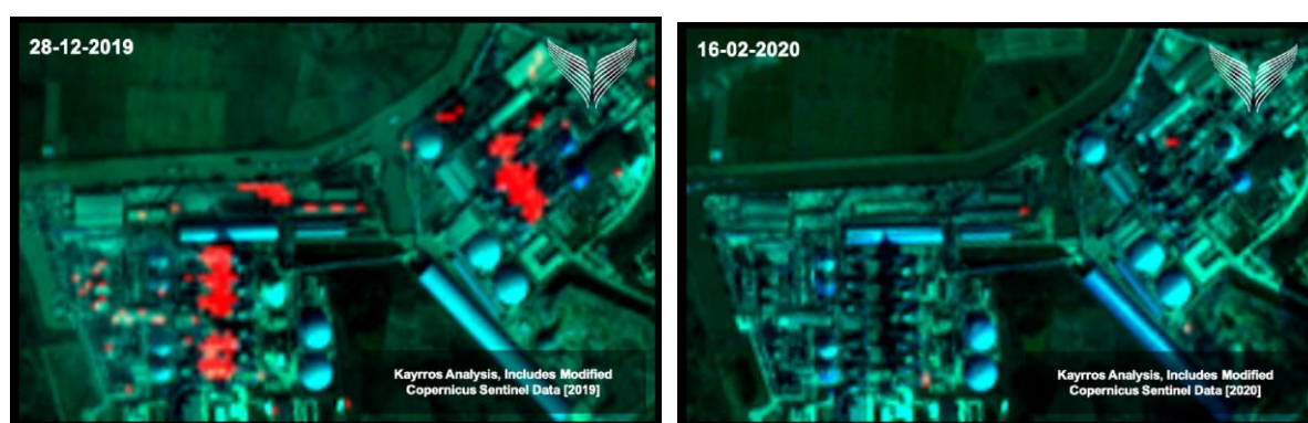
Figure 3. Satellite images of a cement plant in China (LHS: Dec. 2019, RHS: Feb. 2020) Sources: authors, Kayrros SAS
