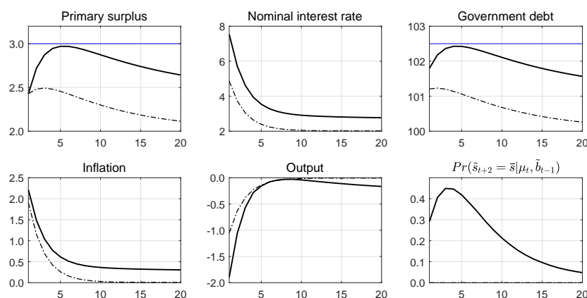
Figure 5: Impulse responses to a cost-push shock
