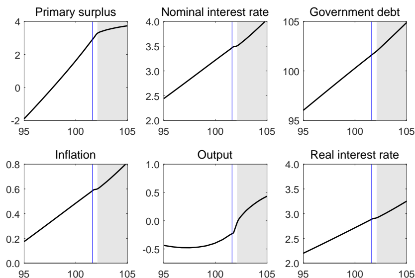
Figure 7: Equilibrium responses to lagged government debt - distortionary taxation
