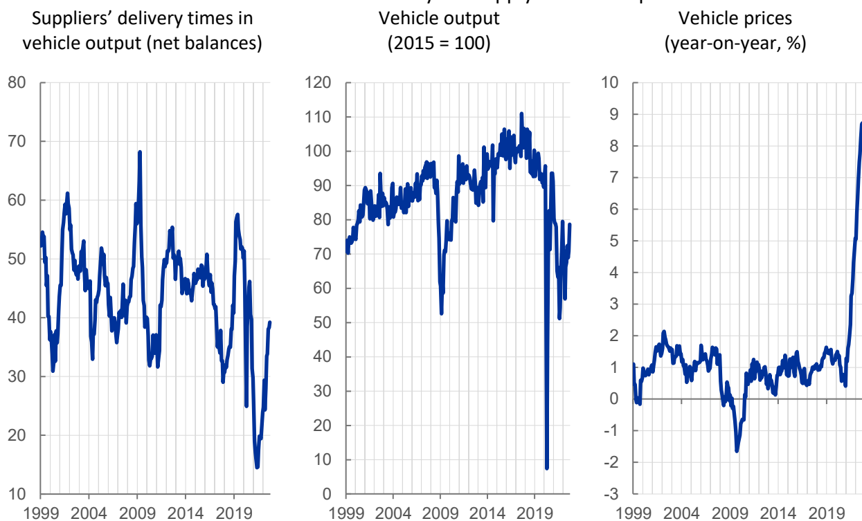
Figure 1: Variables Used to Identify the Great Supply Shocks
