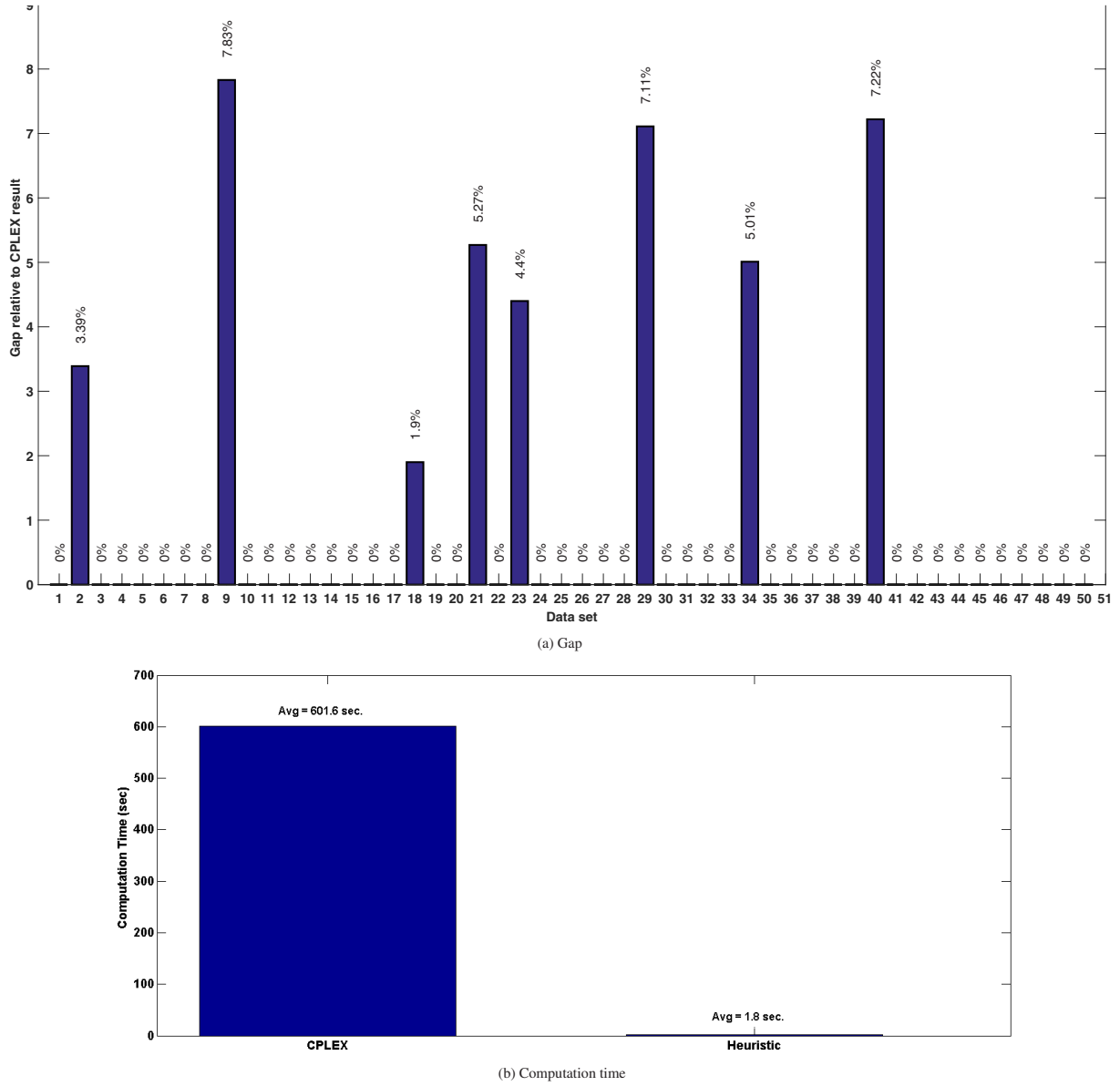
Figure 1: Gap and computation time produced by heuristic for small data sets
