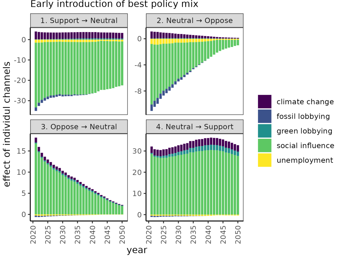
Figure 12: Relative importance of different channels to update opinion in the model including biased assimilation (average of 100 Monte Carlo experiments).
