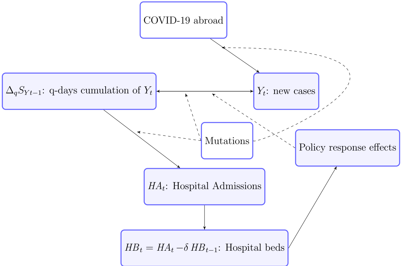
Figure 6: Variables and relationships of CovidMod-STR.
