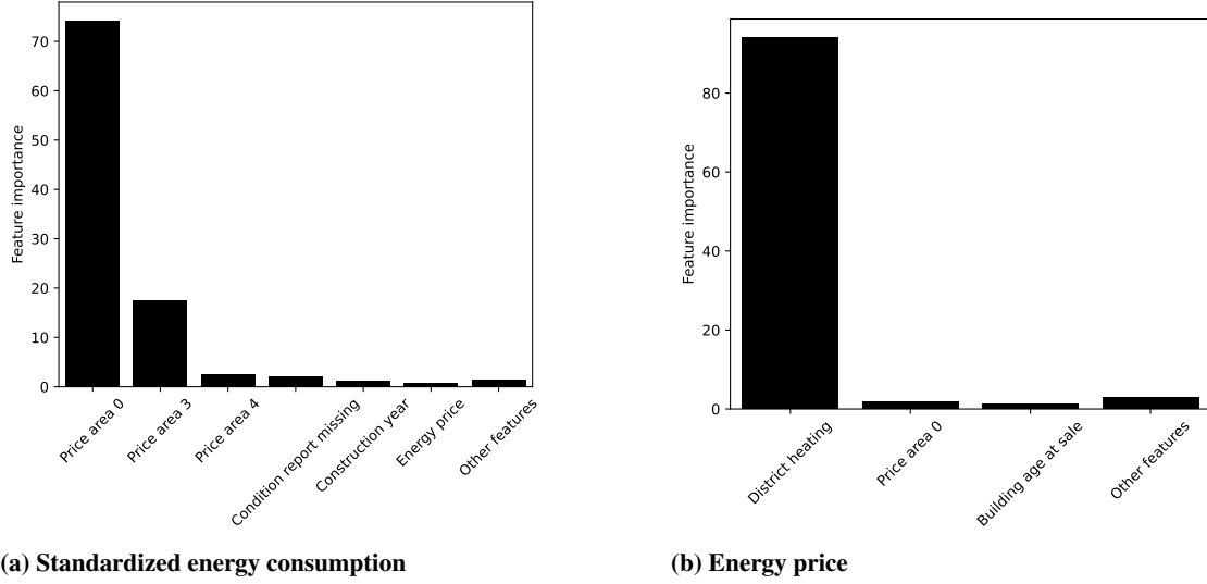
Figure 5 Feature importance
