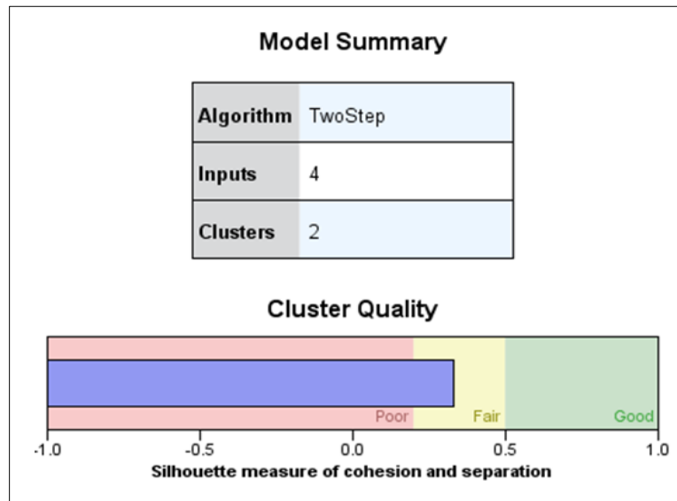
Figure 2: Two-Step Clustering Algorithm Model and Cluster Quality
