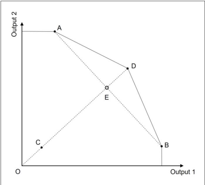
Figure A1: A Simple Illustration of DEA
