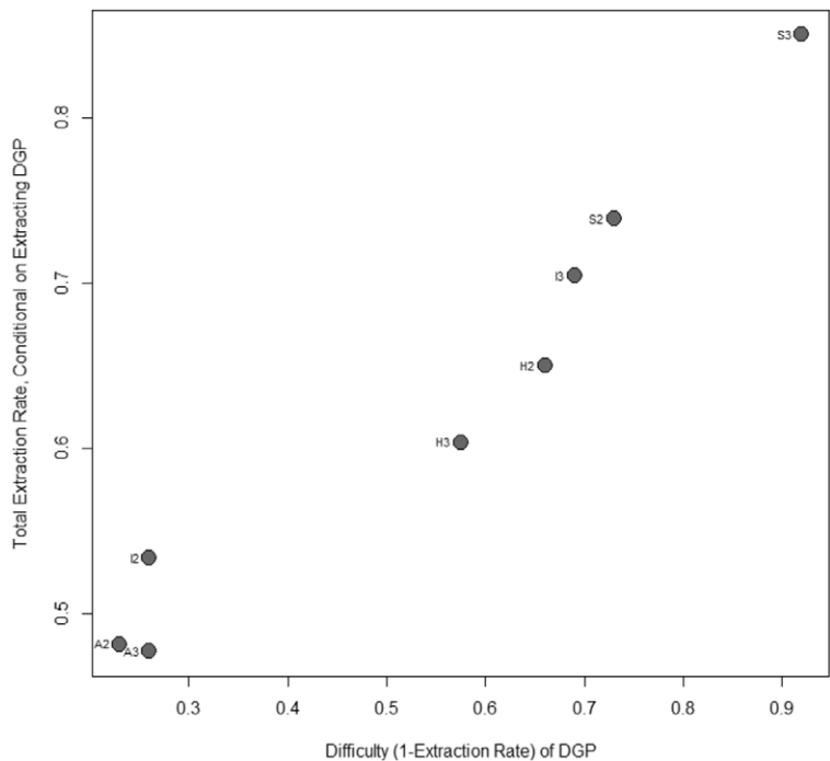
FIGURE 2. Total rate of extraction conditional on extracting a model of each individual DGP. Notes: Data is from 792 choices in the Unique treatment. The x -axis plots the difficulty (one minus the extraction rate) of extracting each DGP, calculated across subjects. The y -axis plots, for each DGP, the average extraction rate (over all DGPs) for the subset of subjects who successfully extracted that DGP.
