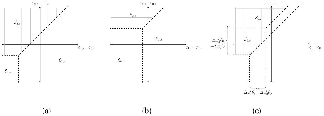
FIGURE 1. Disturbance regions for 3 choices: \Delta x'_2 \theta_0 \geq \Delta x'_1 \theta_0 \geq \Delta x'_0 \theta_0 \implies \mathcal{E}_{2,t} \subset \mathcal{E}_{2,s} .
