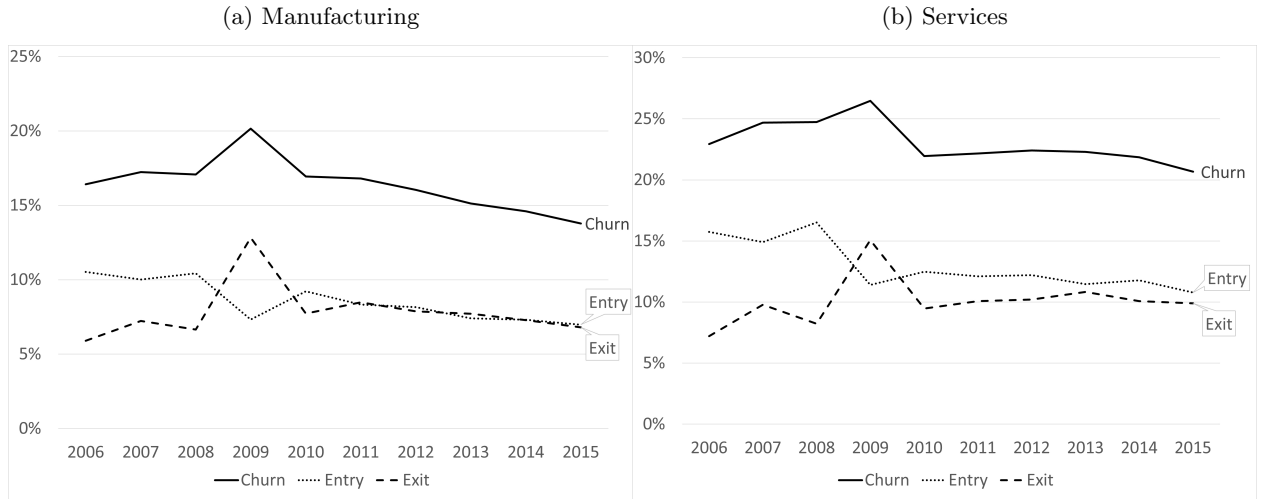
Figure A.2: The entry, exit and churn rates of manufacturing and services industries, 2006-2015
