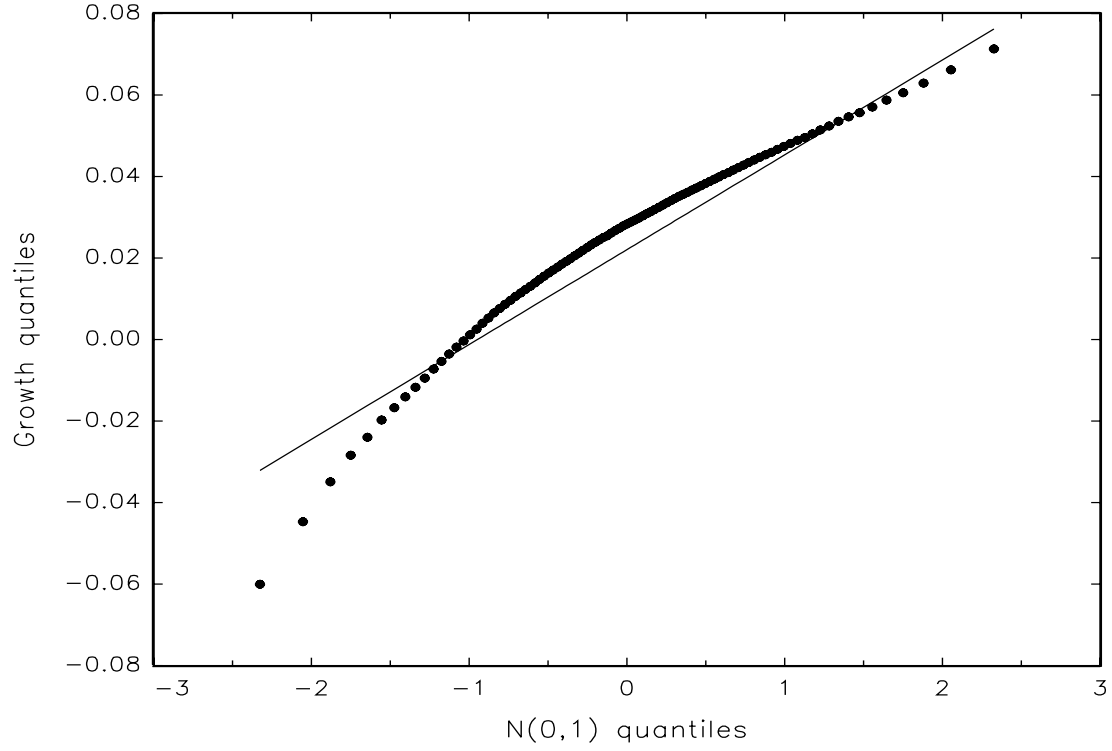
Figure 6. Q-Q plots: \cdots Output growth; — Normal distribution with mean and variance calibrated to output growth
