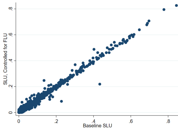
(a) SLU vs SLU Controlled for FLU
