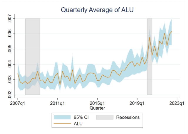
(b) Aggregate Level Uncertainty (ALU)
