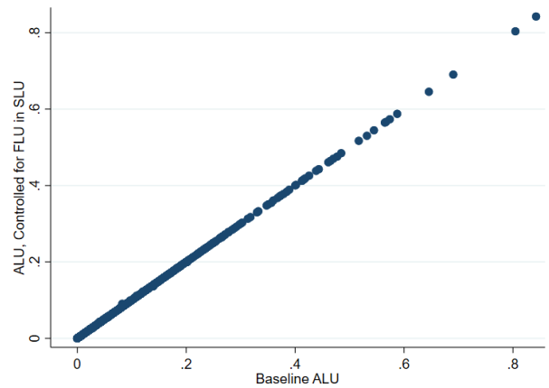
(b) ALU vs ALU Controlled for FLU
