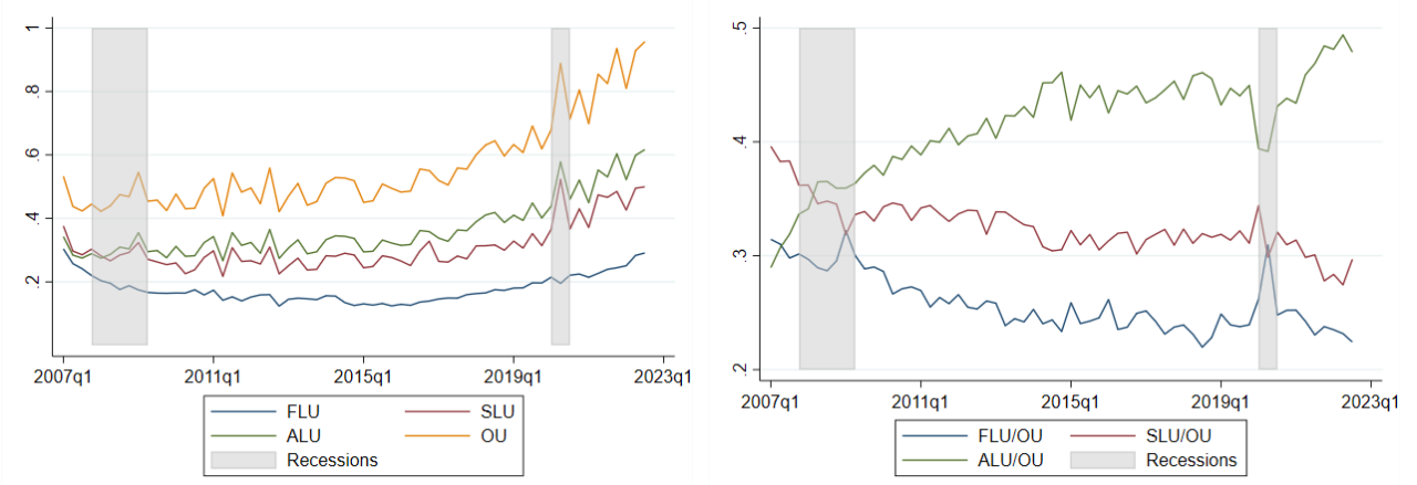
(a) Averaged uncertainty components over time
