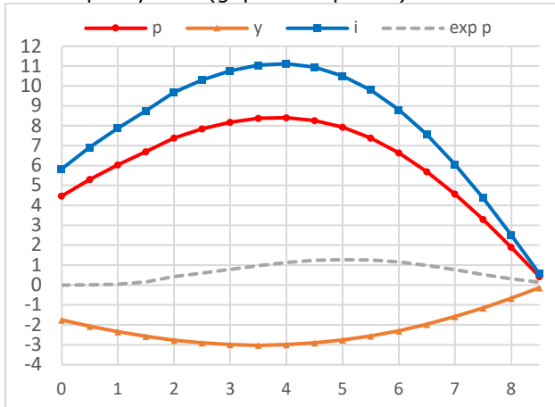
(a) Inflation (p), expected inflation, output and policy rate (gaps in % points)
