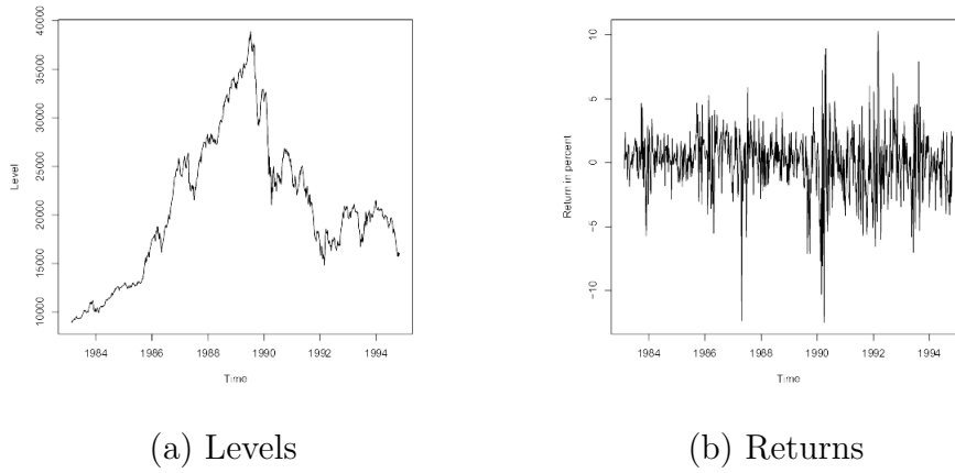
Figure 2: Levels and returns of Nikkei.
