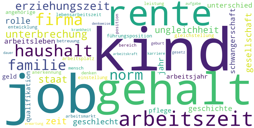
Figure 5: Word-cloud for the full follow-up sample (with grouping)
