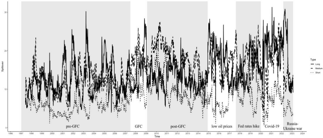
Figure 3: Dynamic frequency connectedness. The solid line represents the frequency connectedness within a long-term horizon defined at d3 \in (20, 200] days, the dashed line represents the frequency connectedness within a medium-term horizon defined at d2 \in (5, 20] days, and the dotted line represents the frequency connectedness within a short-term horizon defined at d1 \in [1, 5] days.
