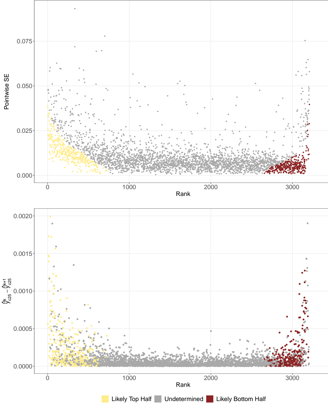
Figure 29: Top Panel for each county we plot the standard error (“SE”) against the rank of the county. Bottom Panel for each county we compute the difference in estimated mobility ( \hat{y}_{c25}^k ) and the next county ( \hat{y}_{c25}^{k+1} ) in the estimated ranking. Next, we plot these differences against the estimated ranks of the counties. Each dot on both panels represents a county. The county is assigned to a high mobility group (light color) if the upper endpoint of its simultaneous confidence set is in the top half of the national ranking. The county is assigned to a low mobility group (red color) if the lower endpoint of its simultaneous confidence set is in the bottom half of the national ranking. Grey colors represent the counties with simultaneous confidence sets such that the places cannot be assigned to either the high or the low mobility group. We emphasize two points: 1) the middle of the ranking does not have particularly large SEs; 2) in the middle of the ranking estimates of mobility are more similar.
