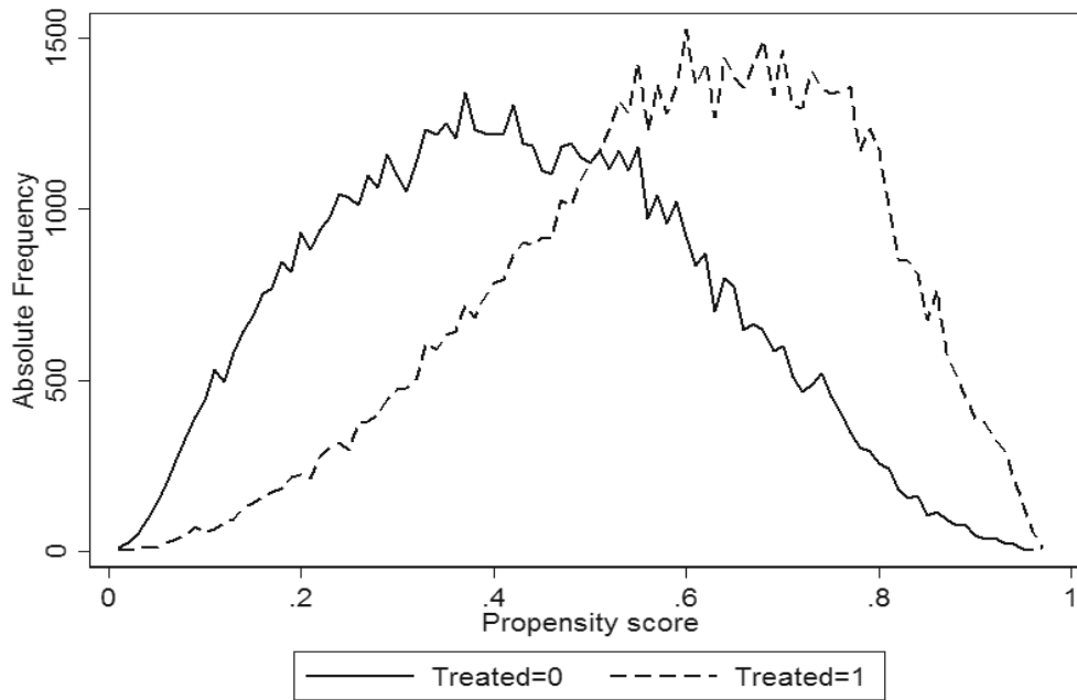
Figure 3: Common Support
