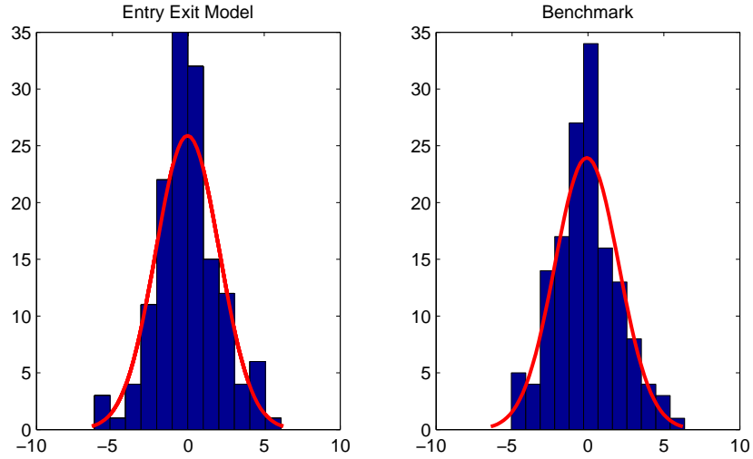
Figure 13: Histograms
