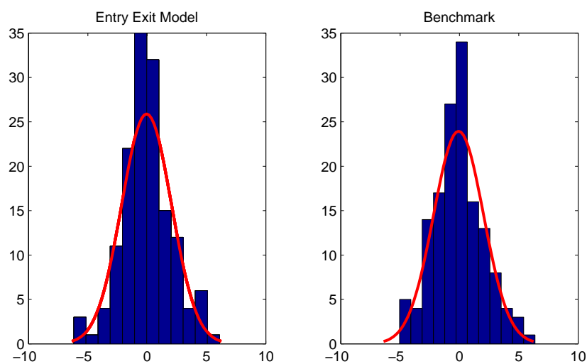
Figure 13: Histograms
