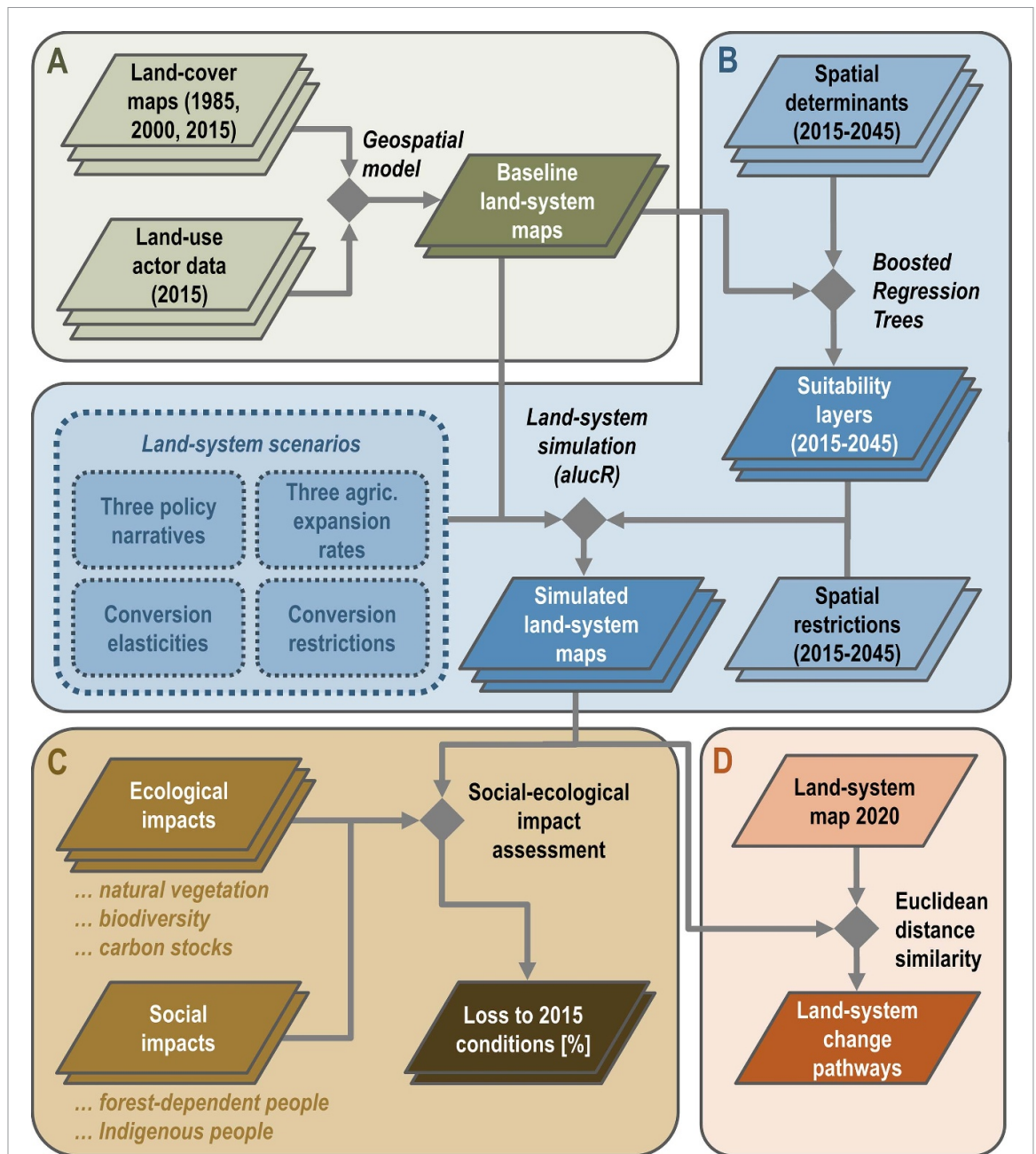
Figure 1. Overview of key processing steps to analyse land-system futures in the Chaco. (A) Land-system mapping, (B) scenario development and land-system simulation, (C) social-ecological impact analyses, and (D) comparison of actual vs. simulated land-system changes. Light colours indicate input data sets, dark colours results, and diamonds analysis steps.
