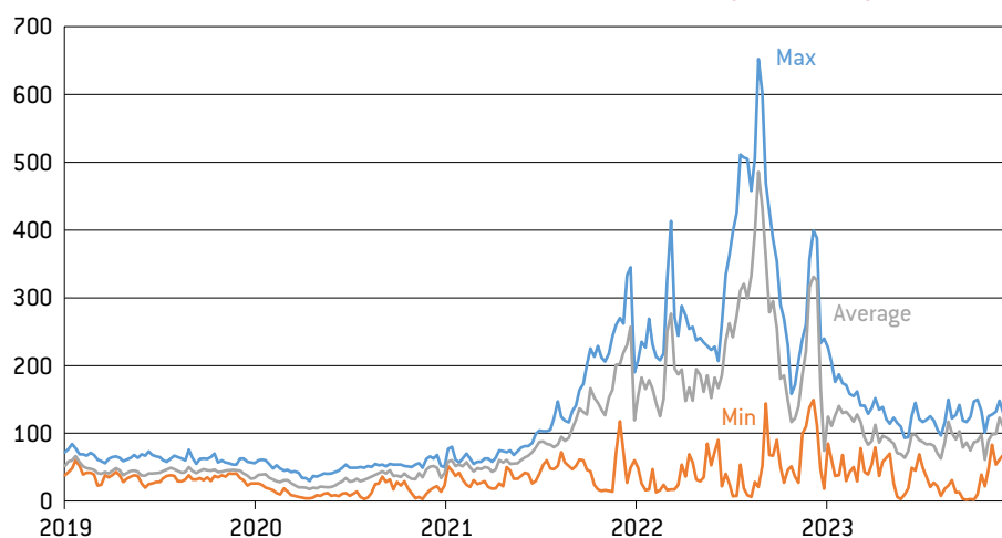
Figure 1: European min, max and average wholesale weekly electricity prices, €/MWh
