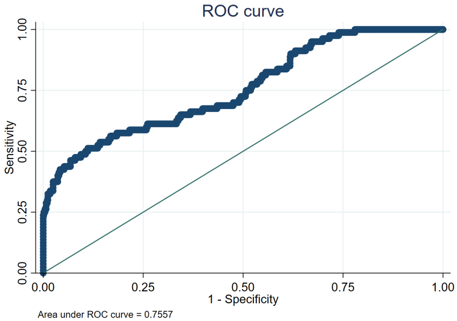
Figure 6: The ROC curve
