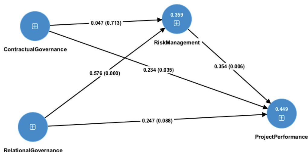
Figure 2. PLS-SEM for project performance.
