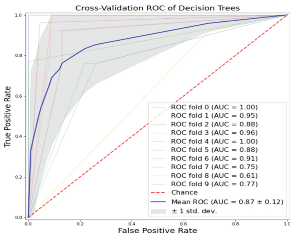
Figure 5. AUROC for decision trees.
