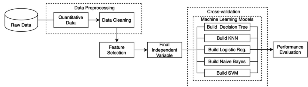
Figure 4. Architecture of proposed model.
