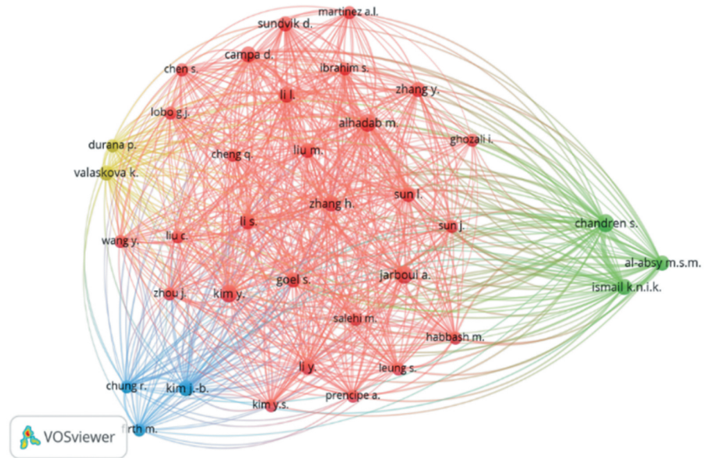
Figure 9. Co-author analysis.
