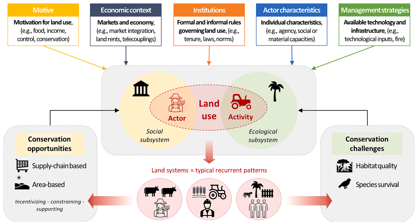
Fig. 3. Conceptual model underlying our land system typology. We regard land systems as integrated social-ecological systems with land use as the link between social processes (via land-use actors) and ecosystem changes (via land-use activities). We consider five groups of interacting factors that shape land use (boxes in the first row). To structure the resulting complexity and diversity of land-use actors, activities, and contexts (second row), we define specific land systems (red circles in the third row) as typical recurring patterns of land-use actors, activities, and social-ecological contexts, translating into specific conservation challenges (threats to species and ecosystems) and opportunities for conservation action. (For interpretation of the references to colour in this figure legend, the reader is referred to the web version of this article.)
