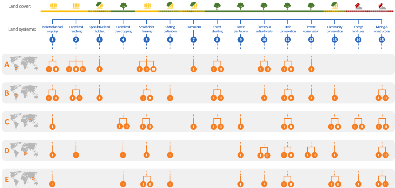
Fig. 4. Scalable land system typology, with 15 general land systems at the highest level, and regionalized systems for five regions: (A) the Gran Chaco dry forest in Argentina, (B) the Chiquitano dry forest in Bolivia, (C) the Deccan dry forests in India, (D) the Miombo-Mopane woodlands in Mozambique, and (E) the Indochina dry forests in Cambodia. The top row demonstrates the limited number of classes that a land-cover perspective would typically identify (cropland, tree cover, built-up, bare soil). See Table 2 for a short description of the associated regional land system. A detailed description of regionalized land systems (i.e., land-use actors and activities) as well as literature references validating the typology is provided in the Supplementary Information 4 .
