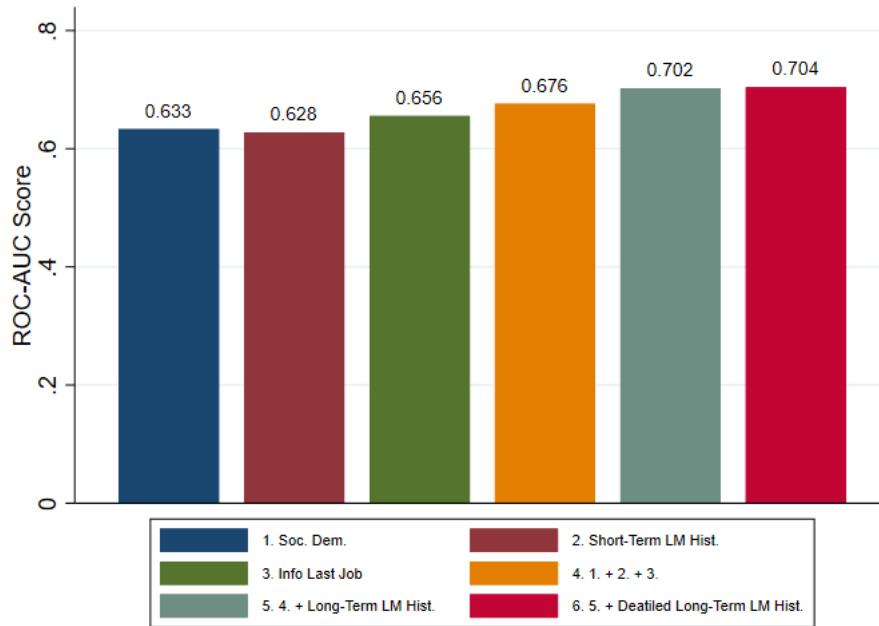
Figure A8: ROC-AUC for different variable inputs – no CW info
