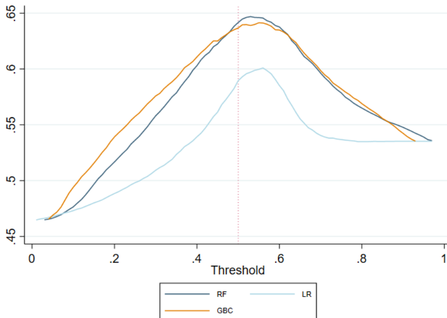
Figure B 4: Accuracy across thresholds by method – admin data 2012/13
