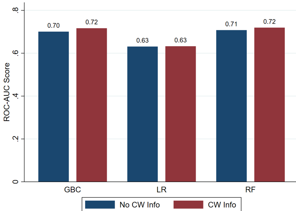
Figure B 3: ROC-AUC by method – admin data 2012/13
