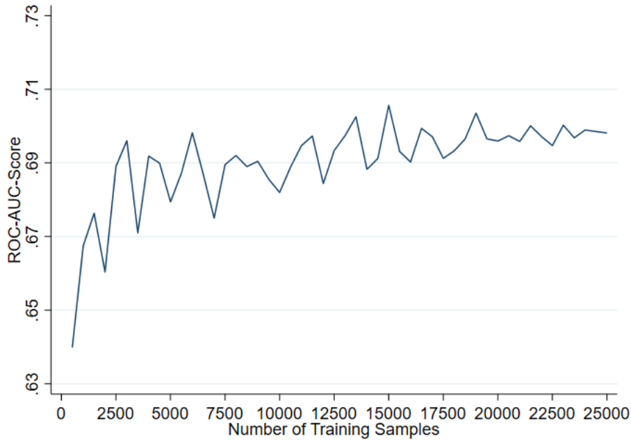
Figure A 10: ROC-AUC Scores for an increasing number of training samples (1000 – 25000 Training Samples)
