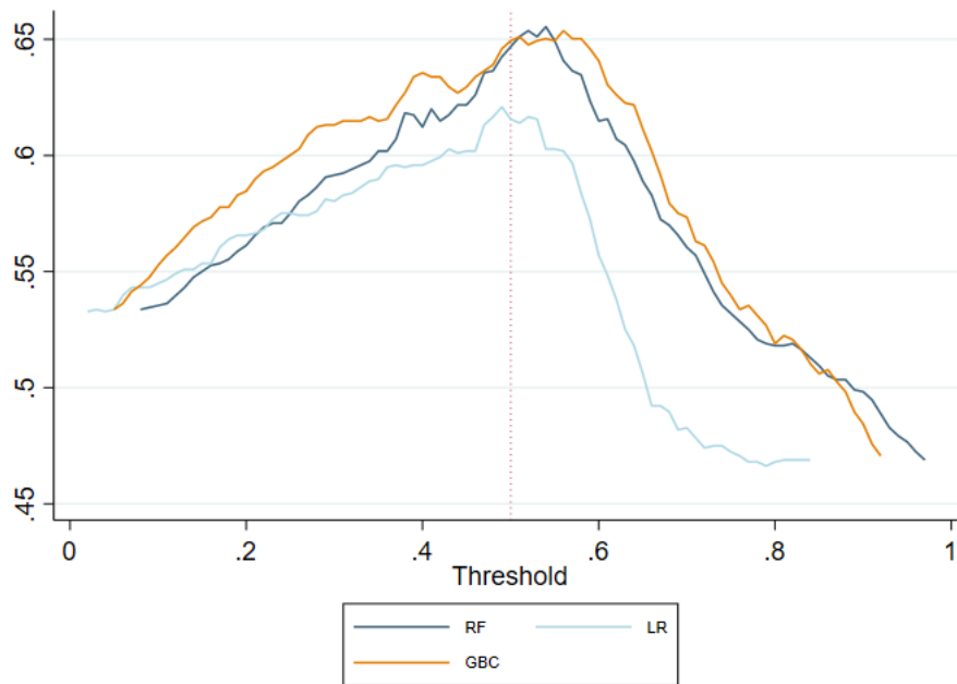
Figure A 12: Accuracy across thresholds by method – survey data
