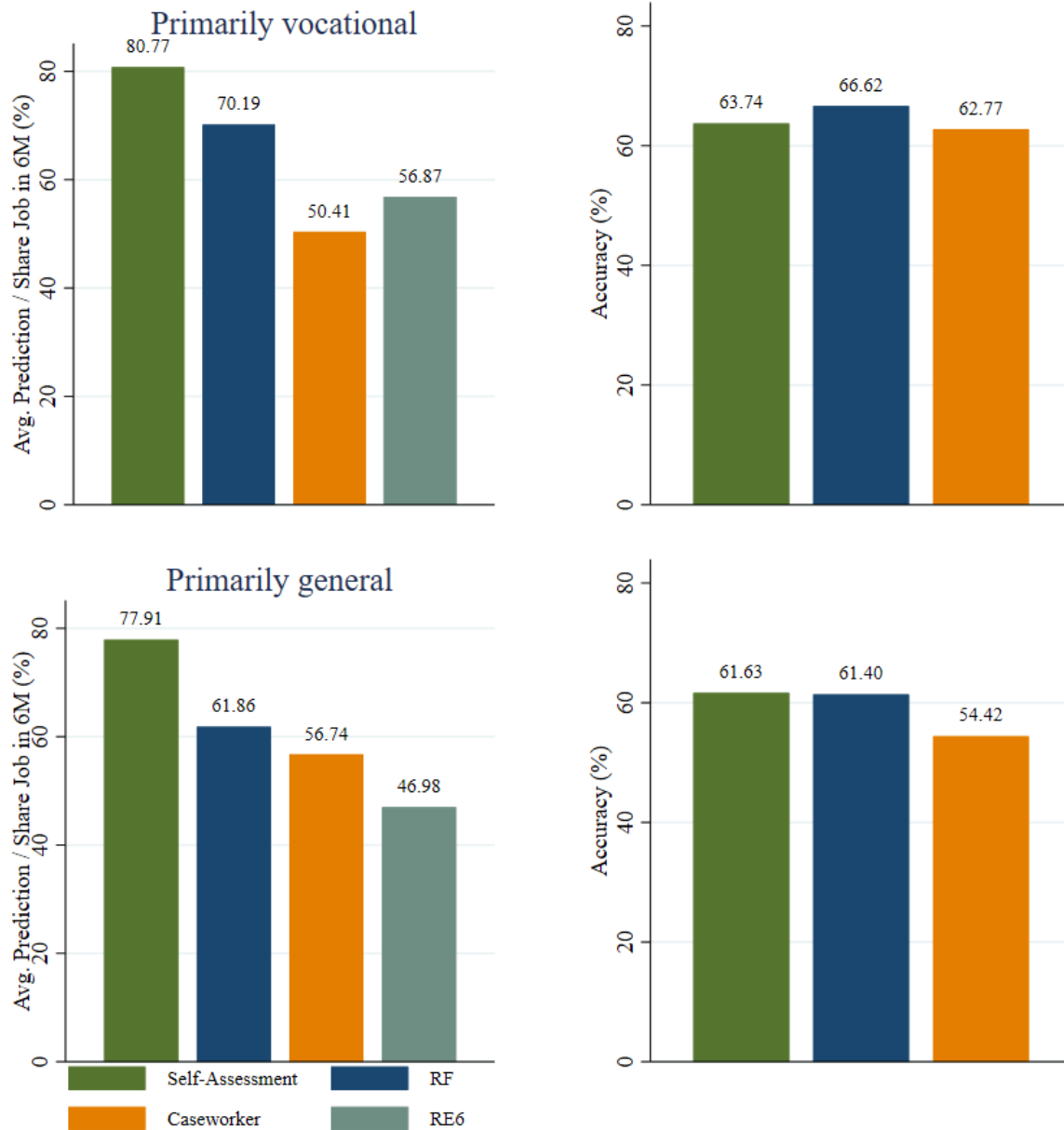
Figure 7: Predictions and accuracies by education
