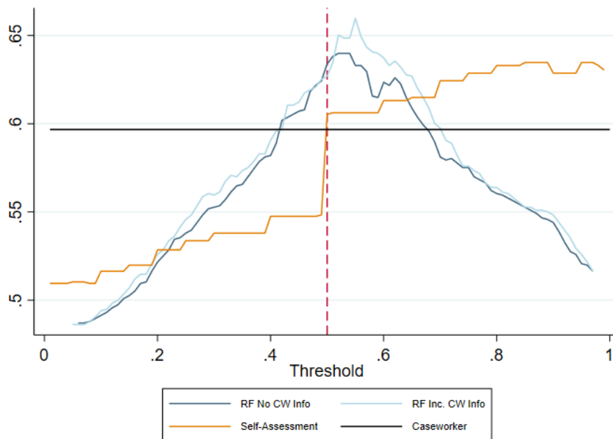
Figure A3: Accuracy of the four predictors across thresholds (outcome “having a job” instead of “finding a job”)
