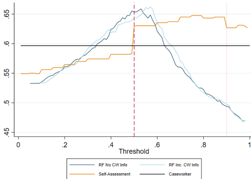
Figure A 13: Accuracy across thresholds using 2012/13 data as training input – survey data
