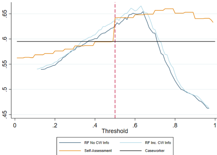
Figure A5: Accuracy of the four predictors across thresholds (less strict sample restrictions)
