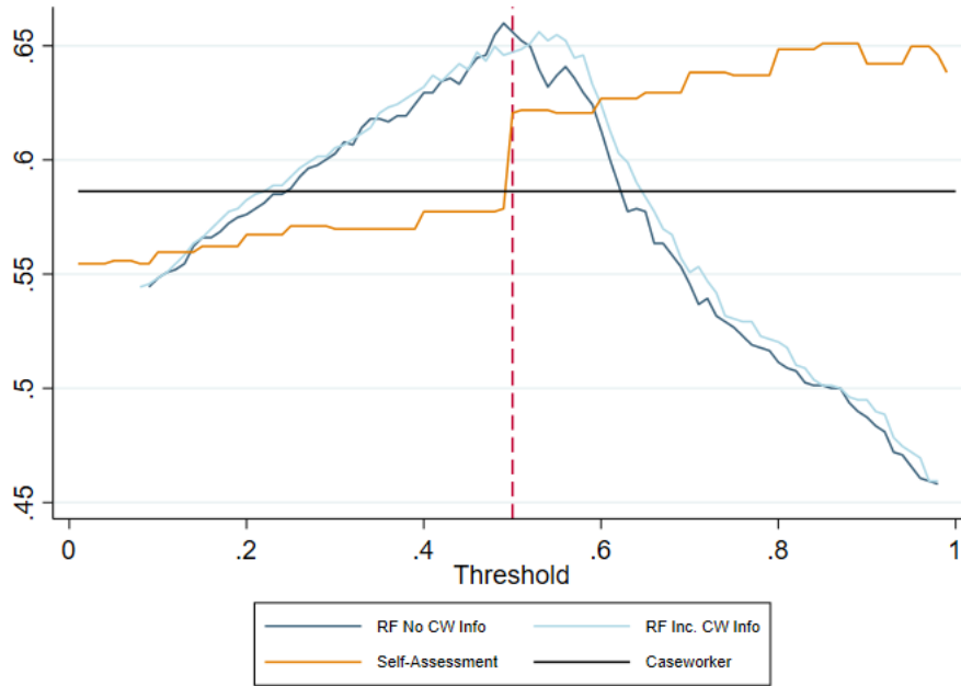
Figure A4: Accuracy of the four predictors across thresholds (profiles not older than 6 weeks)
