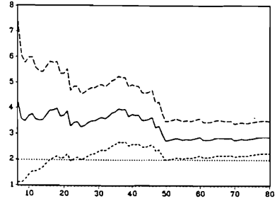
Figure 2. Coefficient of regular variation as a function of q : yen-dollar series
