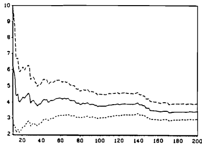
Figure 2. Coefficient of regular variation as a function of q : yen-dollar series
