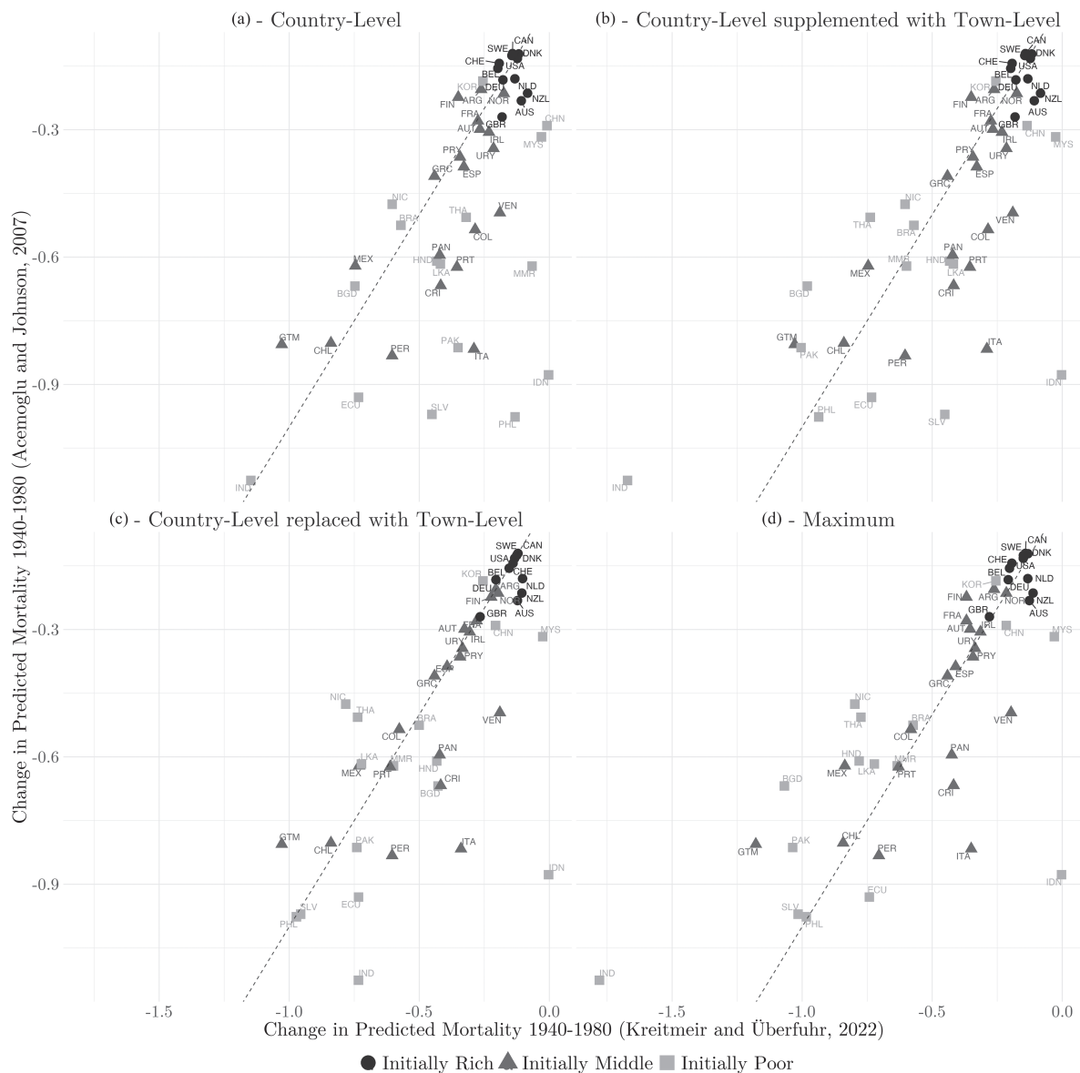
FIGURE 1 Comparison of change in predicted mortality instruments. The sample consists of the 47 baseline countries in AJ . Initially rich, initially middle, and initially poor countries are depicted by black circles, gray triangles, and light-gray squares, respectively. The 45° ray (dashed line) is presented.
