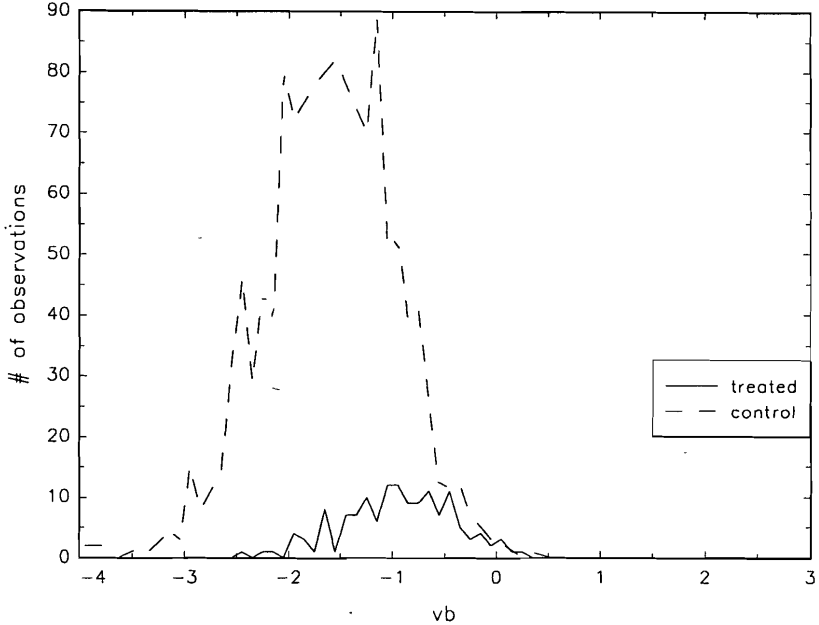
Figure 5: Distribution of v_n \hat{\beta} for OFT and controls
