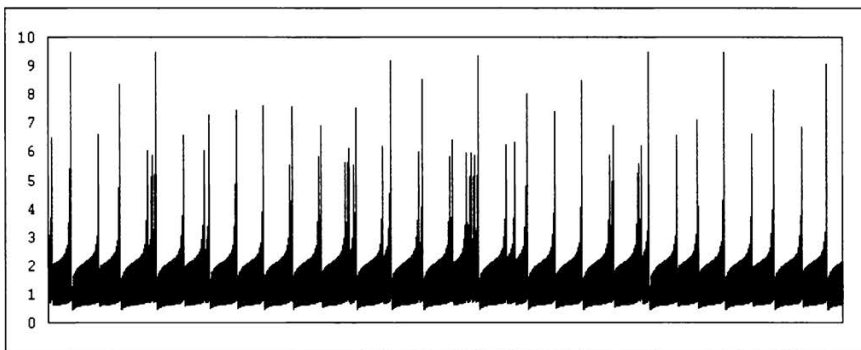
c) \phi = -10, \nu = 50, \iota = 10^4, \chi = \lambda = 0.45, \theta = 0.95, S_{t-3} = 1.00000000, S_{t-2} = 0.99000000, \text{ and } S_{t-1} = 1.02000000 . Data range: 6001 – 10000.
