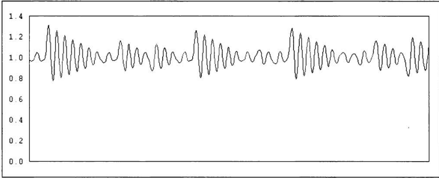
a) \phi = 0, \nu = 500, \iota = 10^4, \chi = \lambda = 200, \theta = 0.95, S_{t-3} = 1.00000000, S_{t-2} = 0.99000000, \text{ and } S_{t-1} = 1.02000000 . Data range: 9900 – 10000.
