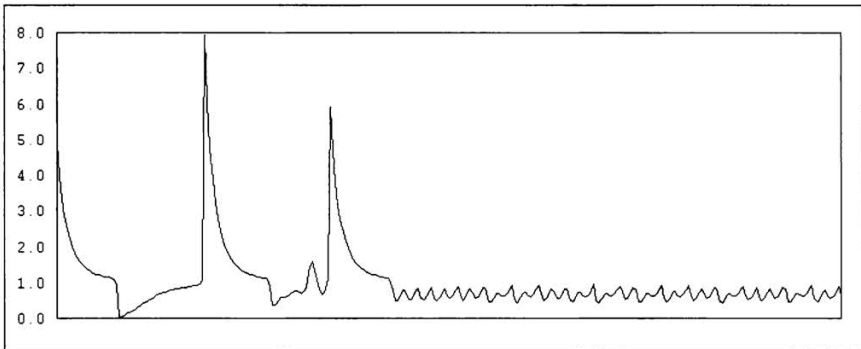
b) \phi = 1, \nu = 500, \iota = 10^4, \chi = \lambda = 0.45, \theta = 1.5, S_{t-3} = 1.00000000, S_{t-2} = 0.99000000, \text{ and } S_{t-1} = 1.02000000 . Data range: 9700 – 10000.
