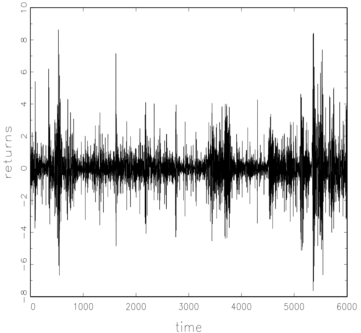
Fig. 1.: A typical ‘realistic’ series of returns from a simulated economy with a binary-coded GA population of 100 agents. For economic parameters, see main text. GA parameters are: p_{\text{mut}} = 0.01 and p_{\text{cross}} = 0.6 .
