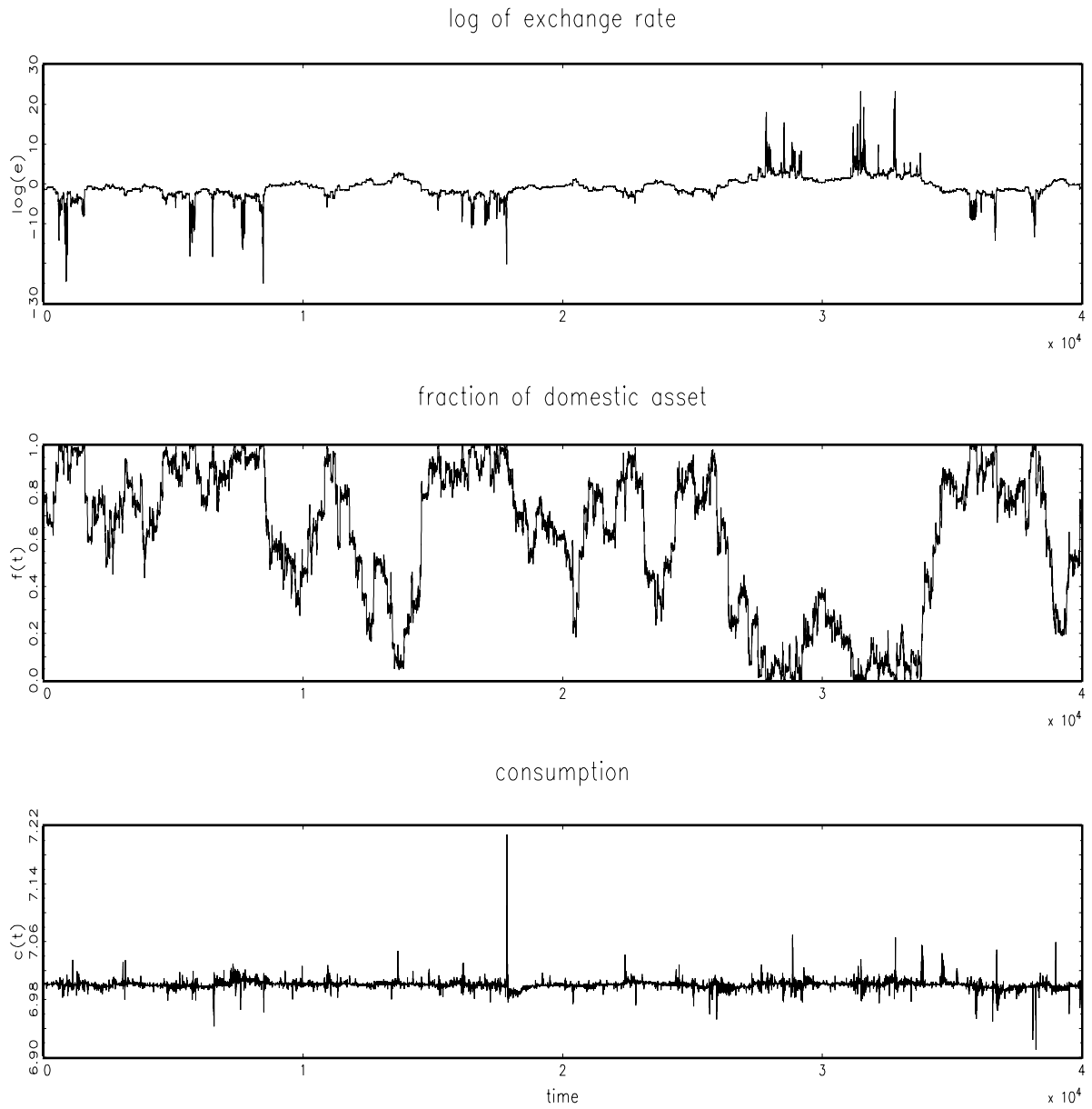
Fig. 3.: Log exchange rate (top), average portfolio fraction of home currency (middle), and average first-period consumption (bottom) for a real-coded GA population of 200 agents. For economic parameters, see main text. GA parameters are: p_{\text{mut}} = 0.05 , \sigma_{\text{mut}} = 0.025 and \gamma = 0.2 . The dynamics seems to be characterized by unsystematic changes of the portfolio composition which lead to exchange rate fluctuations, but leave average consumption choices almost unaffected.
