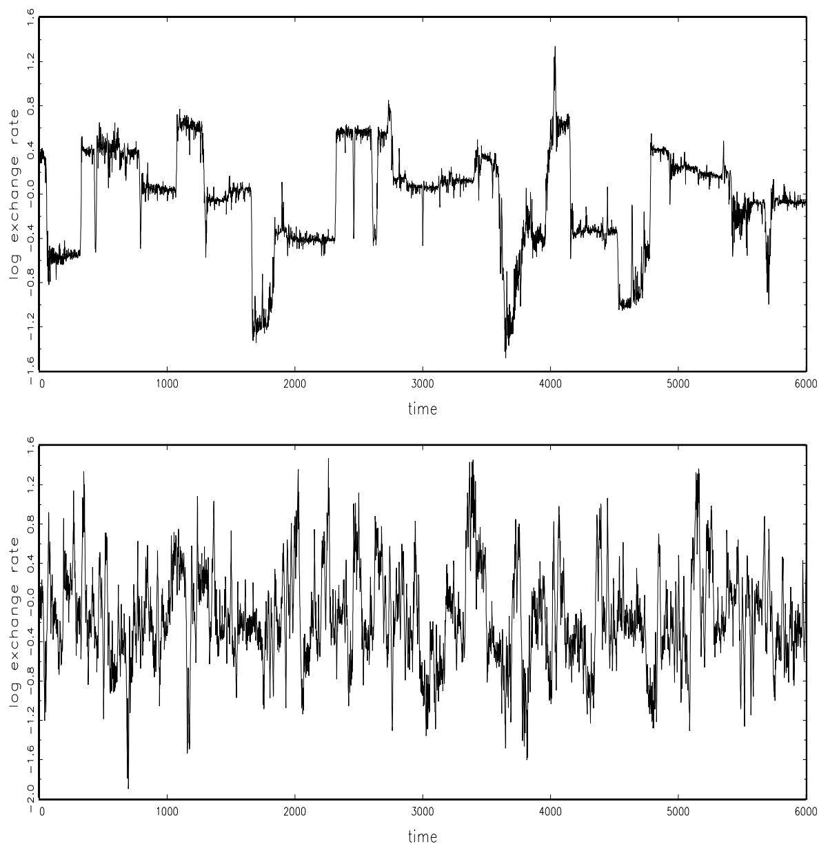
Fig. 2.: Log exchange rates from simulated economies with p_{mut} = 0.01 (upper panel) and p_{mut} = 0.05 (lower panel). The population consists of 100 binary-coded GAs in both cases. Although not fully realistic, for parts of the upper time series the DF and ADF tests are unable to reject the unit root null. The simulation in the lower panel has more easily recognizable mean-reverting features.
