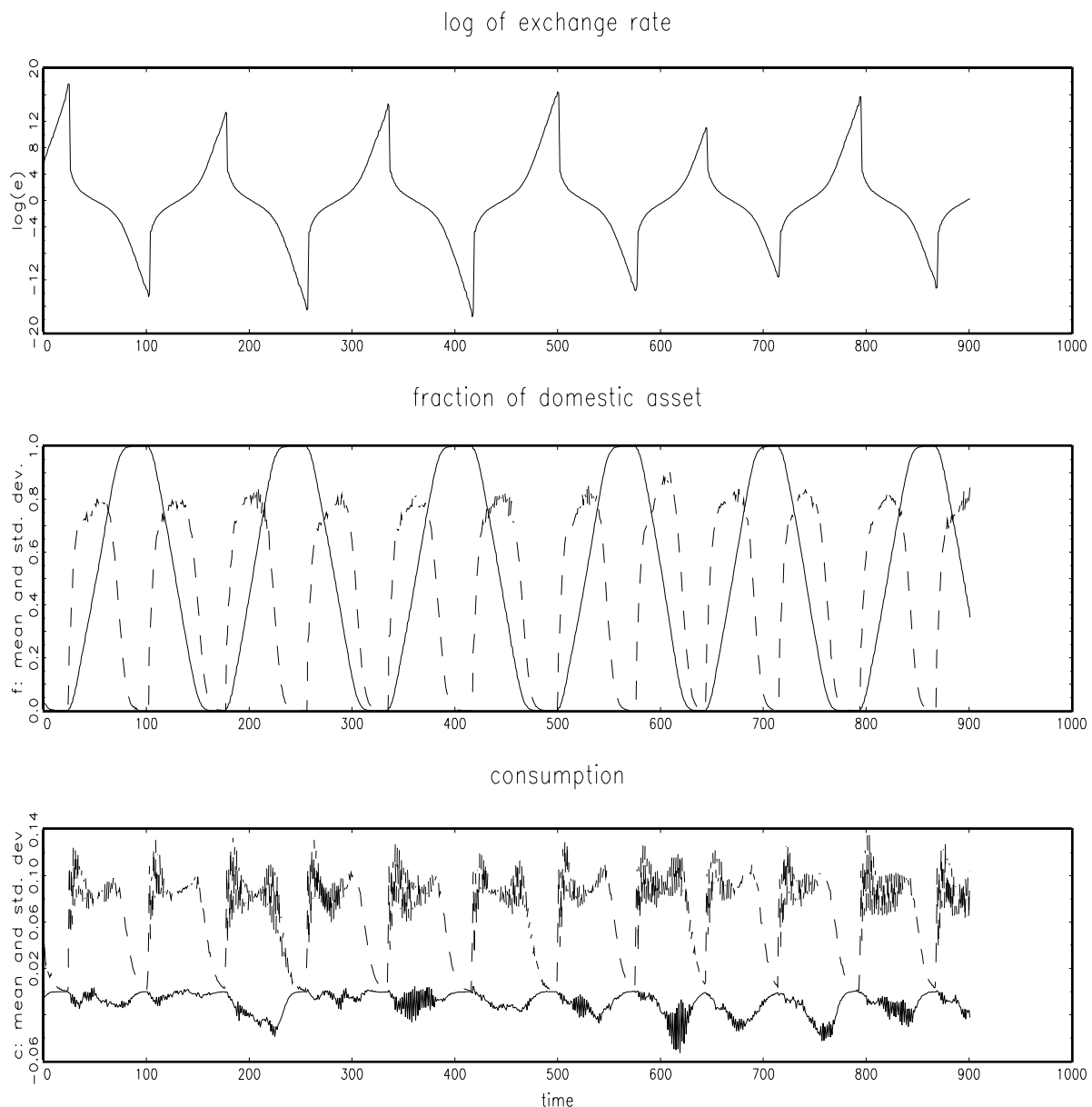
Fig. 4: Log exchange rate (top), average portfolio fraction of home currency (middle), and average first-period consumption (bottom) for a real-coded GA population of 20,000 agents. For economic parameters, see main text. GA parameters are: p_{\text{mut}} = 0.3 , \sigma_{\text{mut}} = 0.025 and \gamma = 0.2 . The middle and bottom panels show both the mean (solid lines) and standard deviations (broken lines) of the distribution of the choice variables within the population. In order to lodge the mean and standard deviation in the bottom panel, we have subtracted the steady state value c^* = 7 , reduced the standard deviation of c_i(t) by one-half and magnified the standard deviation of f_i(t) by a factor 10. The higher p_{\text{mut}} compared to Fig. 3 mainly serves to decrease the amplitude of the cycle and enhance convergence to regular cycles,
