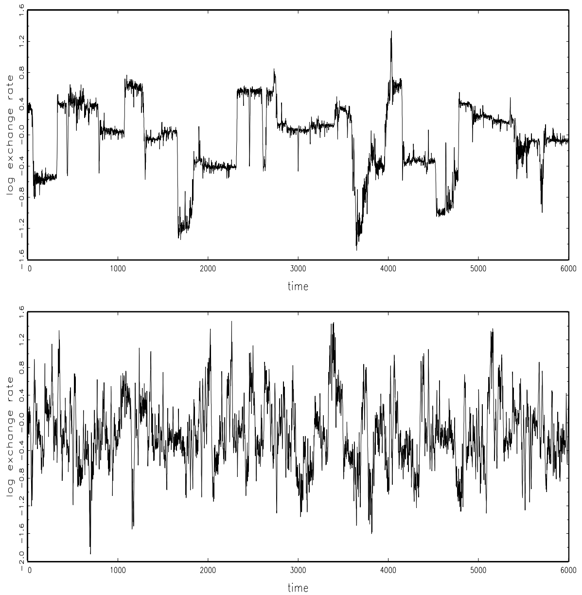
Fig. 2.: Log exchange rates from simulated economies with p_{\text{mut}} = 0.01 (upper panel) and p_{\text{mut}} = 0.05 (lower panel). The population consists of 100 binary-coded GAs in both cases. Although not fully realistic, for parts of the upper time series the DF and ADF tests are unable to reject the unit root null. The simulation in the lower panel has more easily recognizable mean-reverting features.
