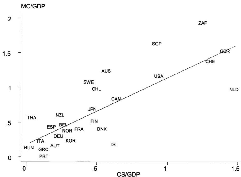
Figure 4: Contractual savings and market capitalization, 1996
