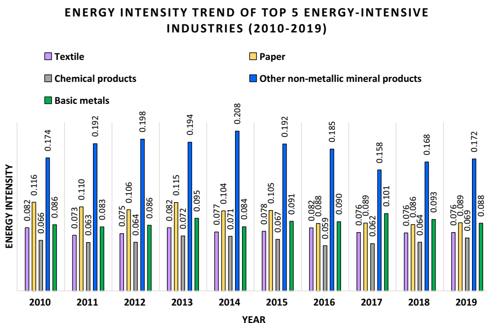
Figure 4.2 Energy intensity trend of five industries from 2010–2019.
