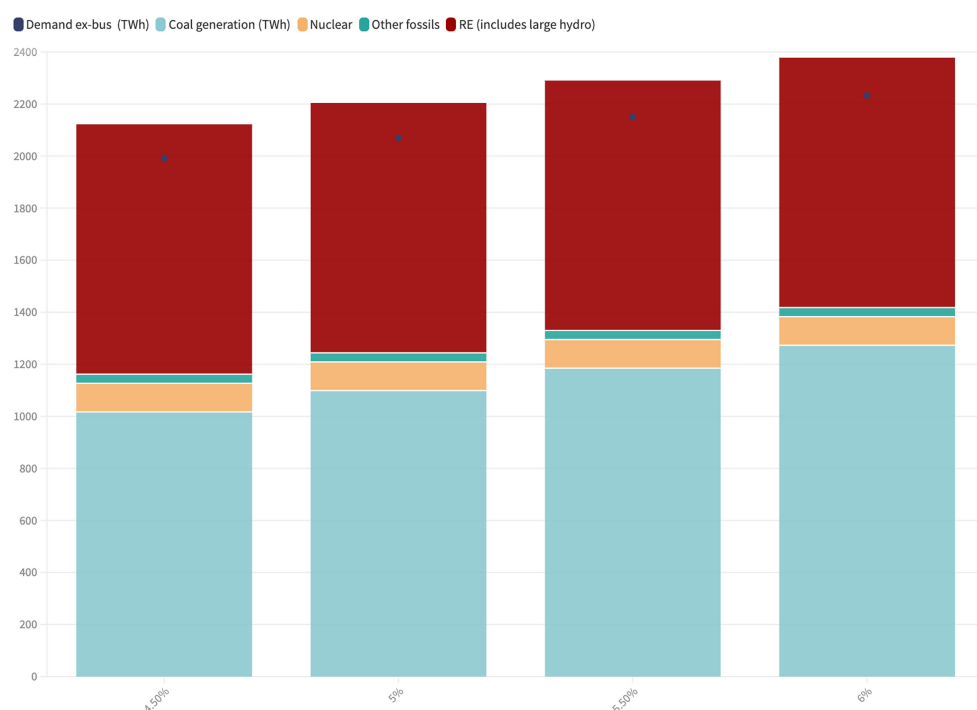
Figure 1.2 Coal-fired generation in FY 2030 under different electricity demand growth scenarios.
