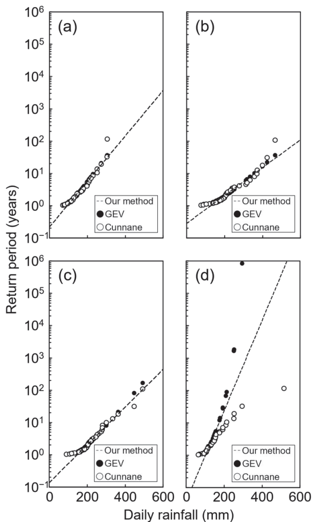
Figure 8. Comparison of RP estimated by the proposed regression equation, RP estimated by the GEV, and RP by the empirical method (Cunnane [39]) at AMeDAS Izumi (a), Morotsuka (b), Aso-Otohome (c), and Asakura (d).
