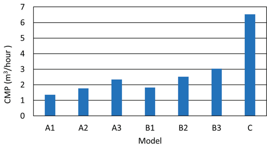
Figure 13. Comparison of the CMP among models for productivity evaluation.
