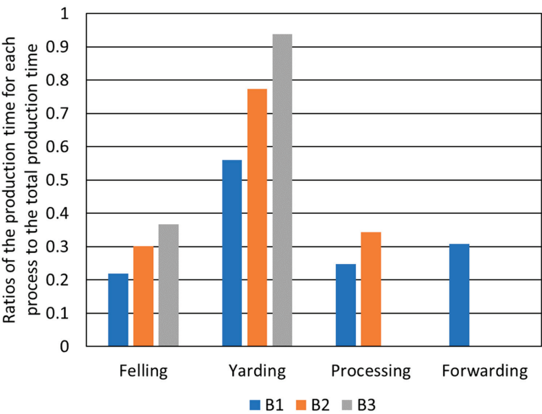
Figure 15. Ratios of the production time for each production process to the total production time for the parallel models.
