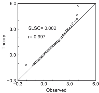
Figure 6. Quantile–quantile plot.
