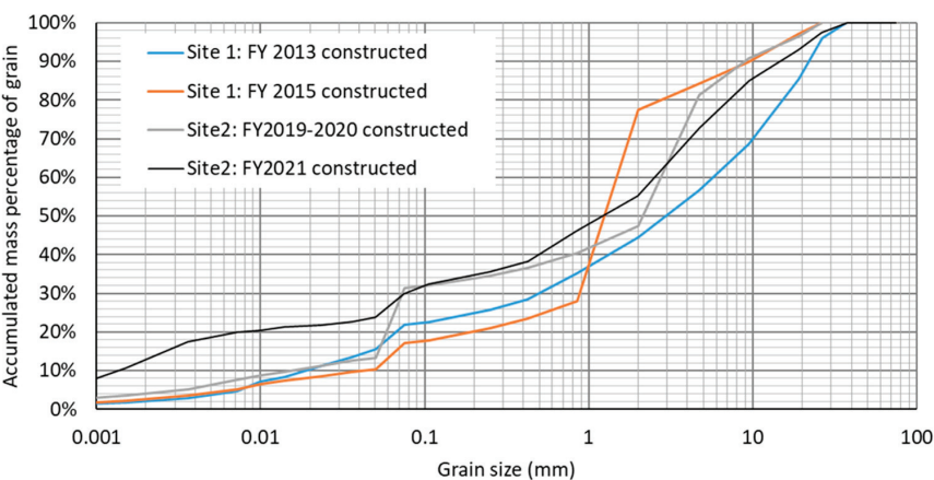
Figure 8. Grain size distribution of soil sampled at Sites 1 and 2.
