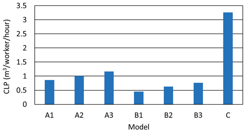
Figure 14. Comparison of the CLP among models for productivity evaluation.
