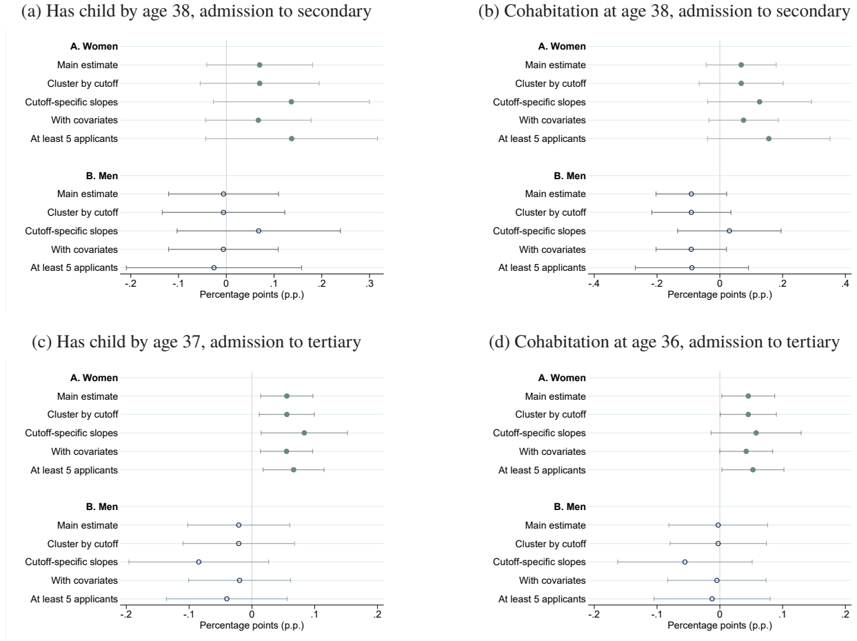
Figure A.11: Robustness to choice of specification
