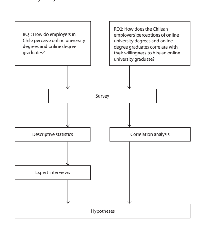
Figure 1 Methodological framework
